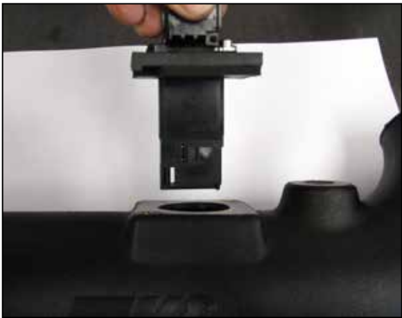
14. Install the mass air sensor assembly into the K&N intake tube so the opening is towards the filter end of the tube. Secure the assembly with the provided hardware.
