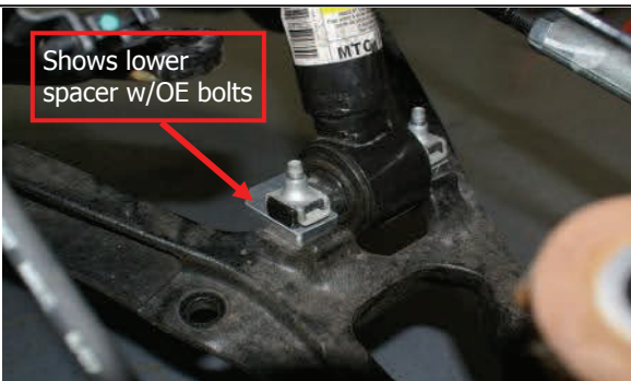
Use new nuts for upper spacer and OE bolts with lower spacer (for 66-3085 kit). Lower not included in 66-3080.
