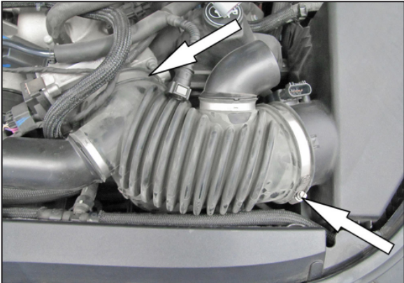
6. Loosen the two hose clamps securing the factory intake tube and remove the intake tube from the vehicle.
