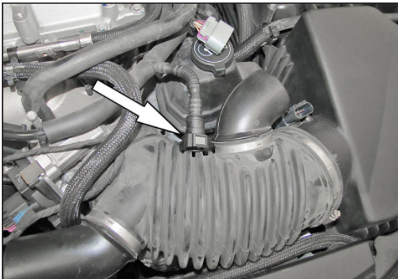
5. Disconnect the crank case vent line from the factory quick disconnect fitting.
