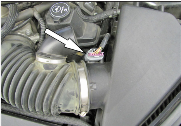
4. Disconnect the mass air sensor electrical connection.
