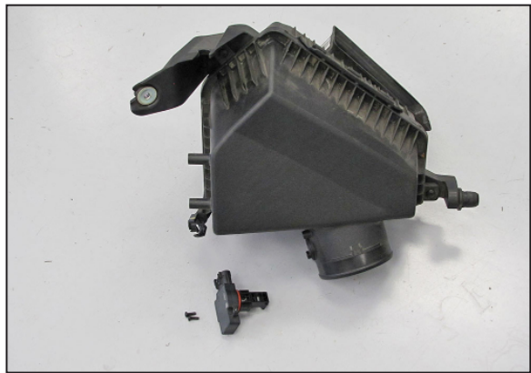
21. Remove the two screws securing the mass air sensor into the factory air filter housing and then remove the sensor from the housing.
