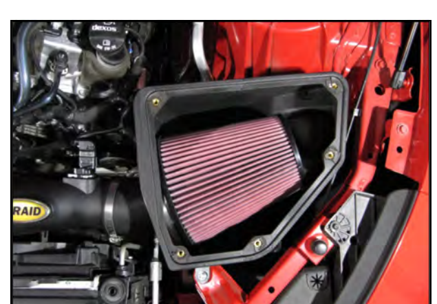
24. Install the Air Filter onto the filter adapter, inside the Airbox.
