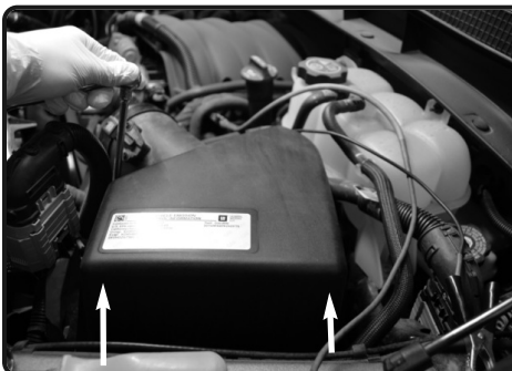
9. Loosen the screws holding in the upper half of the air box. Lift up and remove the upper air box.
